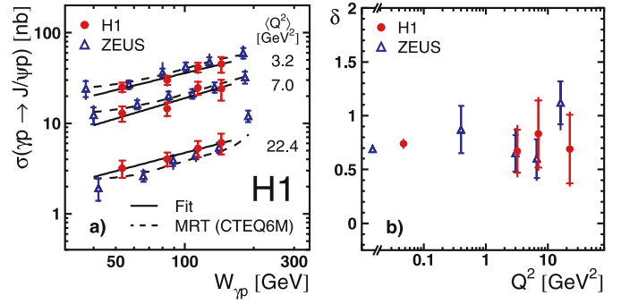
Fig. 6. a Total cross sections for elastic J/\psi production as a function of W_{\gamma p} in the range |t| < 1.2 \text{ GeV}^2 in electroproduction in three bins of Q^2 . \langle Q^2 \rangle indicates the bin centre value in the Q^2 range considered. The solid lines show fits to the H1 data of the form \sigma \propto W_{\gamma p}^\delta . The dashed curves show the MRT QCD prediction based on the gluon distribution CTEQ6M [47] with the normalisation factors from the fit to the Q^2 distribution. Results from the ZEUS experiment [19] in a similar kinematic range are also shown. They have been scaled to the given \langle Q^2 \rangle values using the Q^2 dependence measured by ZEUS. b The fit parameter \delta as a function of Q^2 . The inner error bars show the statistical error, while the outer error bars show the statistical and systematic uncertainties added in quadrature
