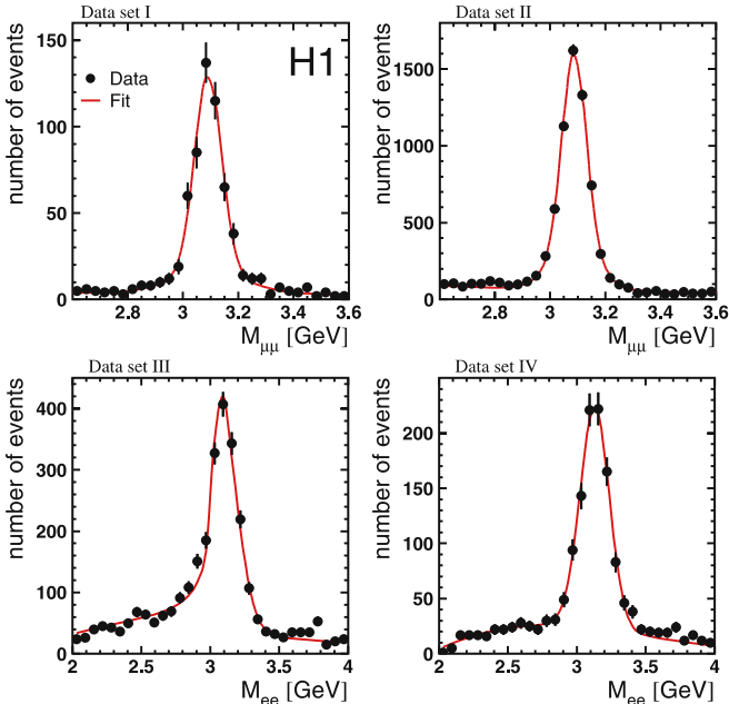
Fig. 2. The dilepton invariant mass distributions (data and fits) in the four kinematic regions defined in Table 1
