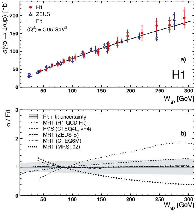
Fig. 5. a Total cross sections for elastic J/\psi production as a function of W_{\gamma p} in the range |t| < 1.2 \text{ GeV}^2 in photoproduction. The inner error bars show the statistical errors, while the outer error bars show the statistical and systematic uncertainties added in quadrature. The solid line shows a fit to the H1 data of the form \sigma \propto W_{\gamma p}^\delta . Results from the ZEUS experiment [6] in a similar kinematic range are also shown. b The ratio of theoretical predictions to the fit to the H1 data in a . The shaded band represents the uncertainties of the fit result. Predictions from MRT QCD calculations [8] and a dipole model (FMS, [9]) based on different gluon distributions [47–51] are shown. For the MRT curves the normalisation factors determined from the Q^2 distributions are used. The FMS prediction is normalised to the fit result at W_{\gamma p} = 90 \text{ GeV}
