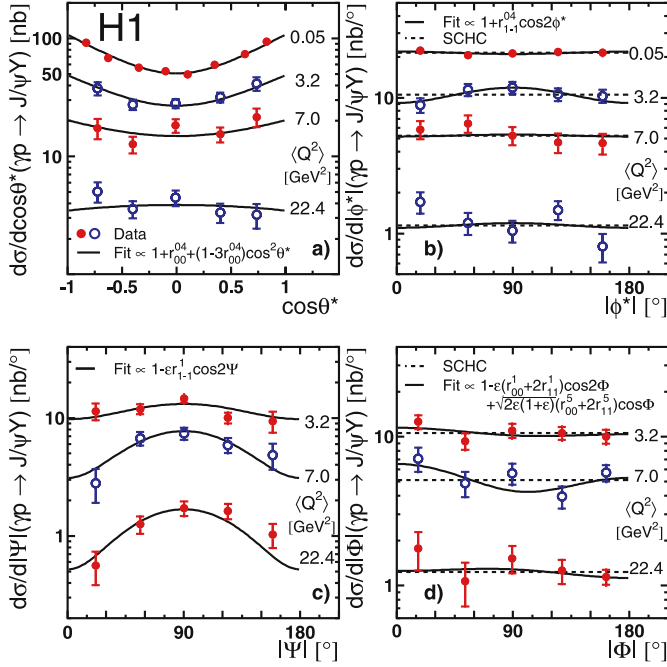
Fig. 11. The differential cross sections for diffractive (elastic and proton dissociative) J/\psi production as functions of the four angles \theta^* , \phi^* , \Psi and \Phi defined in the text. The data are shown in bins of Q^2 for the range 40 < W_{\gamma p} < 160 GeV and |t| < 5 GeV ^2 . \langle Q^2 \rangle indicates the bin centre value in the Q^2 range considered. The inner error bars show the statistical error, while the outer error bars show the statistical and systematic uncertainties added in quadrature. The solid lines represent the results of fits to the data. The dashed lines in b and d are fits assuming s -channel helicity conservation
