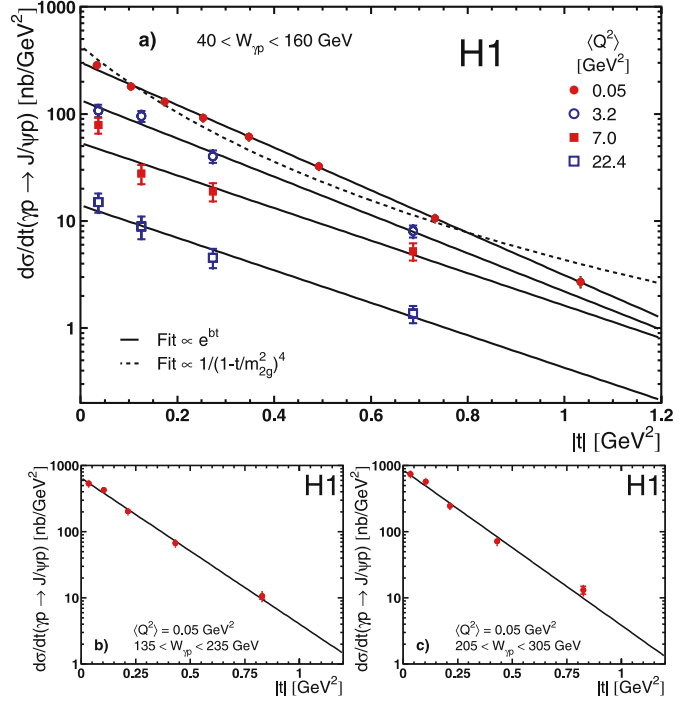
Fig. 7. Differential cross section d\sigma/dt for elastic J/\psi production as a function of |t| a in four bins of Q^2 in the range 40 < W_{\gamma p} < 160 GeV. \langle Q^2 \rangle indicates the bin centre value in the Q^2 range considered. The inner error bars show the statistical error, while the outer error bars show the statistical and systematic uncertainties added in quadrature. The solid lines show fits to the data of the form d\sigma/dt \propto e^{bt} . The dashed curve shows the result of a fit proposed by Frankfurt and Strikman [11]. Figures b and c show the photoproduction measurements in the ranges 135 < W_{\gamma p} < 235 GeV and 205 < W_{\gamma p} < 305 GeV
