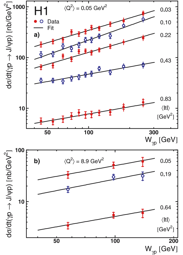
Fig. 8. Differential cross section d\sigma/dt for elastic J/\psi production as a function of W_{\gamma p} in bins of |t| a in photoproduction and b in electroproduction. \langle Q^2 \rangle and \langle |t| \rangle indicate the bin centre values in the ranges considered. The inner error bars show the statistical error, while the outer error bars show the statistical and systematic uncertainties added in quadrature. The solid lines show the results of one-dimensional fits of the form \sigma \propto W_{\gamma p}^{4(\alpha(\langle t \rangle)-1)} in each t bin
