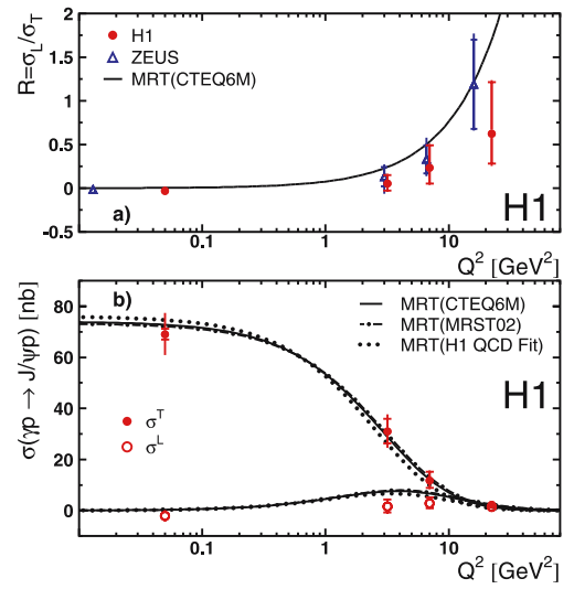
Fig. 13. a Ratio R = \sigma^L/\sigma^T as a function of Q^2 for the range 40 < W_{\gamma p} < 160 GeV and |t| < 5 GeV 2 . The data are compared with the result of a MRT calculation [8] based on the CTEQ6M [47] gluon distribution. Also shown are results from the ZEUS collaboration [6, 19]. b The cross sections for longitudinally and transversely polarised photons \sigma^L and \sigma^T as a function of Q^2 . The MRT QCD calculations based on different gluon distributions ([47–49]) are also shown with the same normalisation factors as derived from Fig. 3. The inner error bars show the statistical errors, while the outer error bars show the total errors
