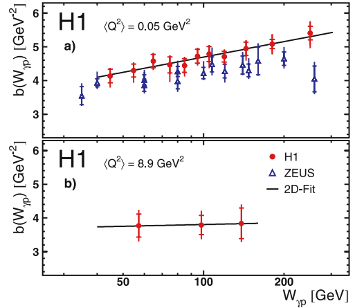
Fig. 10. The values of the t slope parameter b(W_{\gamma p}) as a function of W_{\gamma p} in the range |t| < 1.2 GeV ^2 for a photoproduction and b electroproduction. \langle Q^2 \rangle indicates the bin centre value in the Q^2 range considered. The data points are the results of one-dimensional fits of the form d\sigma/dt \propto e^{bt} in W_{\gamma p} bins. The inner error bars show the statistical errors, while the outer error bars show the statistical and systematic uncertainties added in quadrature. The solid lines show the results of the two-dimensional fits of (2) as in Fig. 8. In a the data are compared with results from the ZEUS collaboration [6]
