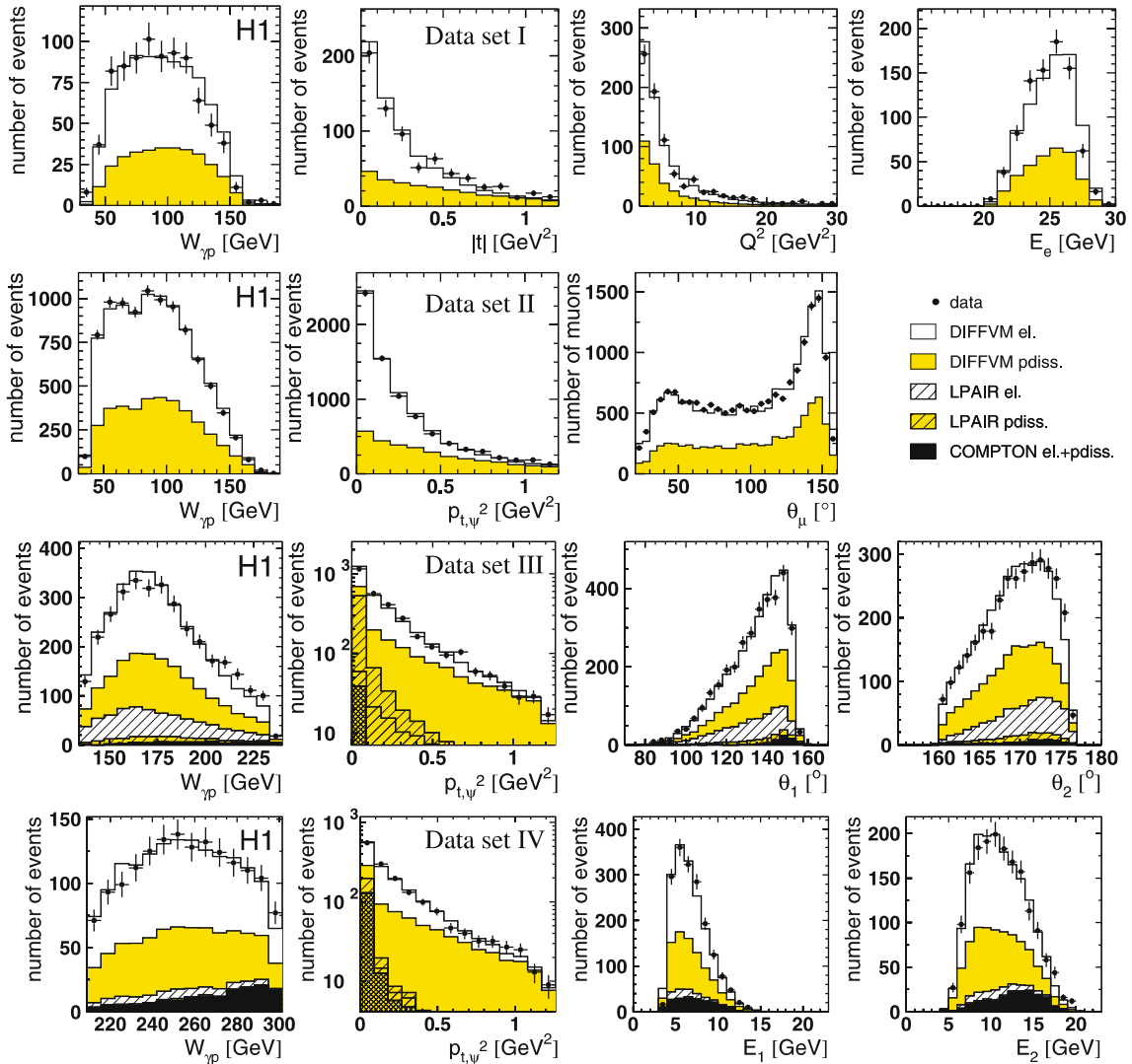
Fig. 3. Observed event distributions for the four data sets ( points ) defined in Table 1, omitting the forward detector cuts against proton dissociative events and in the first two rows omitting the final W_{\gamma p} cuts in the W_{\gamma p} distributions. The first two rows correspond to the selected J/\psi \rightarrow \mu^+\mu^- candidates where the small non-resonant background has been subtracted. The data are shown with the elastic (signal) simulations (DIFFVM el., white area ) and proton dissociation MC (DIFFVM pdiss., shaded area ). Rows three and four correspond to J/\psi \rightarrow e^+e^- candidates, where the non-resonant background is not subtracted. Here, in addition to the elastic and proton dissociative J/\psi simulations the contributions from \gamma\gamma \rightarrow e^+e^- (LPAIR) and Compton scattering (COMPTON) are shown. The normalisations are obtained from a fit of the overall mass peak of each data set. The variables W_{\gamma p} , Q^2 , t and p_{t,\psi}^2 are defined in the text. \theta_\mu refers to the decay muons of data set II. In row three \theta_1 and \theta_2 refer to the decay electrons which are selected in different polar angular regions. In row four E_1 and E_2 refer to the energies of the decay electrons
