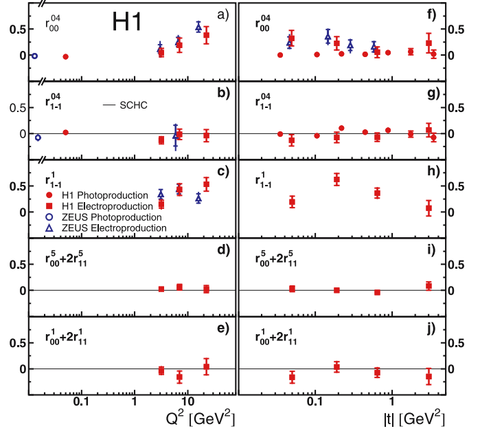
Fig. 12. Spin-density matrix elements as functions of Q^2 a – e and |t| ( f – j ) for the range 40 < W_{\gamma p} < 160 GeV. The data points are the results of fits of equations 4–7 to the data shown in Fig. 10. The inner error bars show the fit result including only the statistical error, while the outer error bars also include the systematic uncertainties. The expectations from SCHC are shown as solid lines . The results from the ZEUS collaboration are also shown, a , c and f [6, 19] and b [5, 18]
