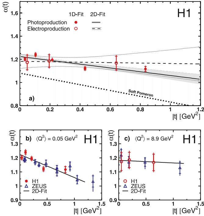
Fig. 9. a The effective trajectory \alpha(t) as a function of |t| in the range 40 < W_{\gamma p} < 305 GeV for photoproduction ( \langle Q^2 \rangle = 0.05 GeV ^2 ) and 40 < W_{\gamma p} < 160 GeV for electroproduction ( \langle Q^2 \rangle = 8.9 GeV ^2 ). The data points are the results of the one-dimensional fits shown in Fig. 7. The inner error bars show the statistical error, while the outer error bars show the statistical and systematic uncertainties added in quadrature. The solid and dashed lines show the results of two-dimensional fits of (2) together with 1\sigma -error bands, which take the correlation between the fit parameters into account. A comparison with the results of the ZEUS collaboration [6, 19] is shown in b and c for photoproduction and electroproduction respectively. The data in [19] are derived at slightly different values of \langle Q^2 \rangle . The lines are results from the two-dimensional fits
