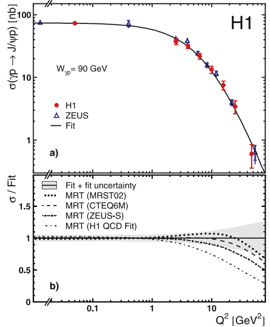
Fig. 4. a Total cross section for elastic J/\psi production as a function of Q^2 in the range |t| < 1.2 GeV 2 at W_{\gamma p} = 90 GeV. The inner error bars show the statistical errors, while the outer error bars show the statistical and systematic uncertainties added in quadrature. The solid line is a fit to the H1 data of the form \sigma_{\gamma p} \propto (M_\psi^2 + Q^2)^{-n} . Data from the ZEUS experiment [6, 19] are also shown. b The ratio of the MRT calculations [8] to the fit from a . The MRT QCD predictions are based on different gluon distributions [47–50]. The curves are individually normalised to the measurements across the complete Q^2 range yielding factors between 1.5 and 2.8. The shaded band represents the uncertainty of the fit result
