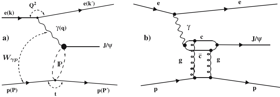
Fig. 1. Elastic J/\psi production, a in an approach based on Pomeron (IP) exchange and b in a pQCD approach via two gluon exchange. The kinematic variables are indicated in a
